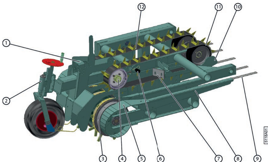
Fig. 18: Pick-up
